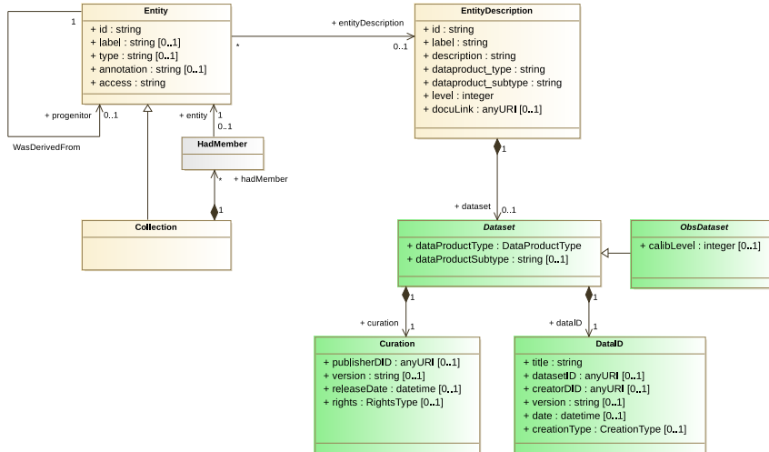
Figure 4: The relation between Entity, Dataset and Collection (see Section 2.2.2). The Dataset class as well as the classes with green boxes belong to the IVOA Dataset Metadata Model. Some attributes of Dataset actually link to Entity-attributes, see Section 3 for more details.
