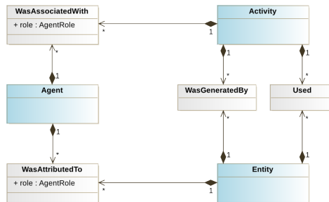
Figure 3: The main core classes and relations of the Provenance Data Model, which also occur in the W3C model.
