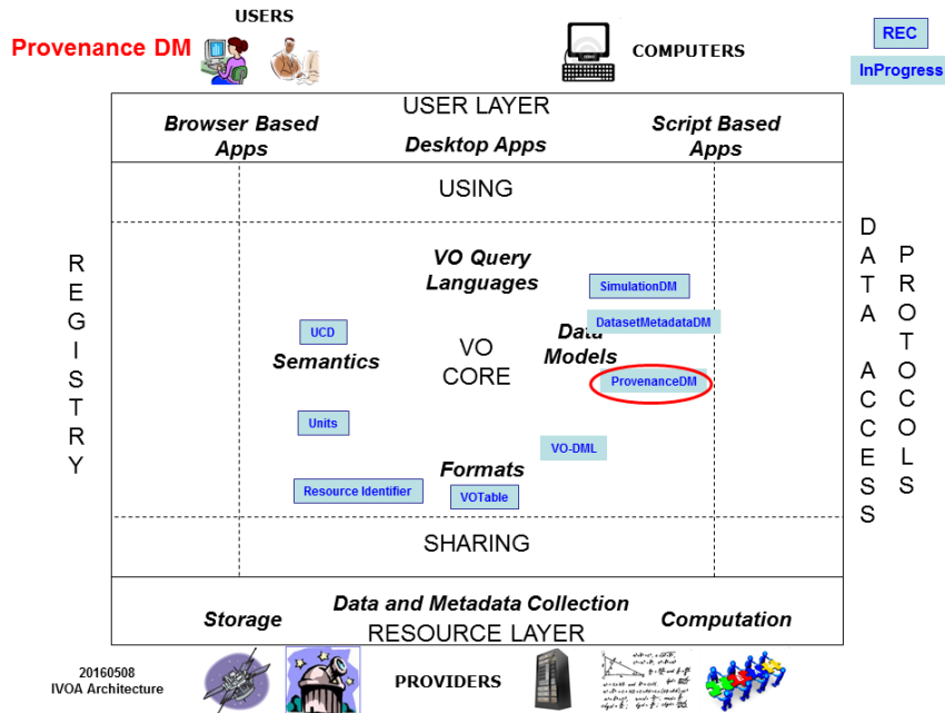
Figure 1: Architecture diagram for the Provenance Data model. It is based on existing concepts defined in existing IVOA data models, and existing formats and semantics and fully integrated in the IVOA framework
