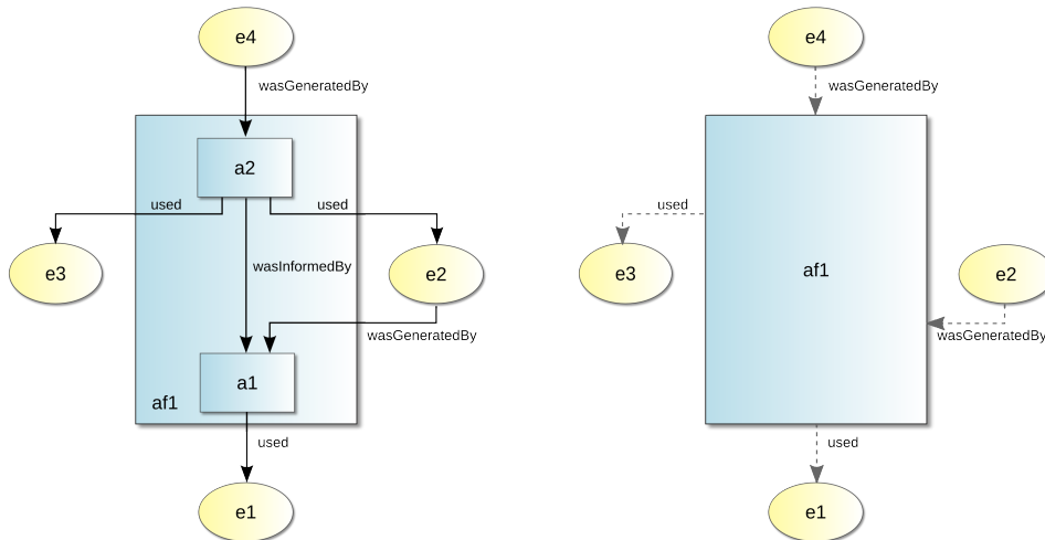
Figure 6: An example provenance graph. The detailed version is shown on the left side. It also shows the shortcut WasInformedBy to connect two activities, which could be used if the entity e2 would not be needed anywhere else. An ActivityFlow can be used to “hide” a part of the provenance graph as is shown on the right side. Activities are marked by blue rectangles, entities by yellow ellipses.
