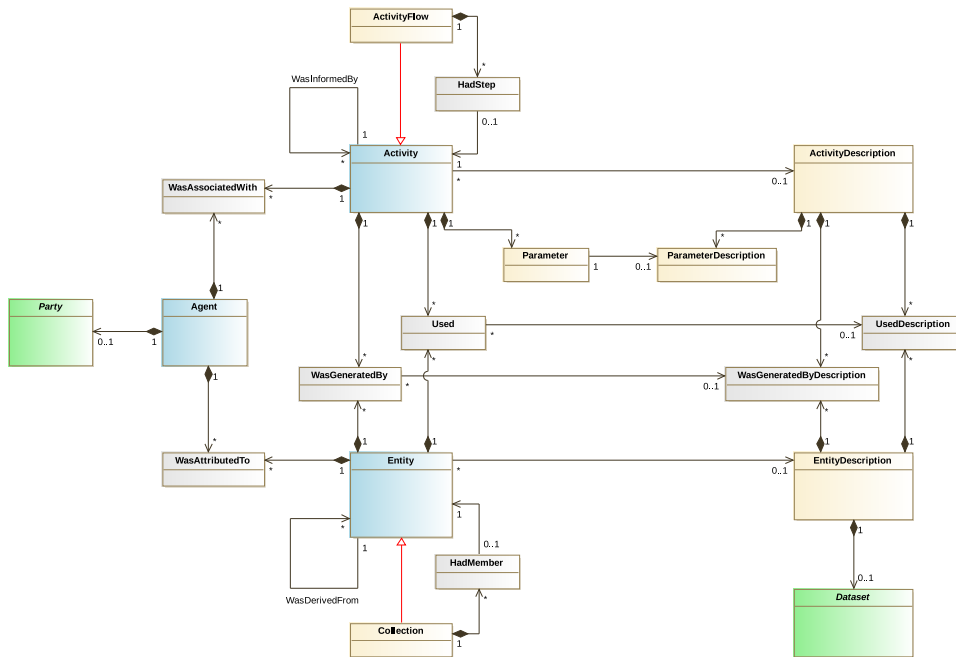
Figure 2: Overview of the classes for the Provenance Data Model in a class diagram. The blue classes are core elements. Green classes are links to the IVOA Dataset Metadata Model.
