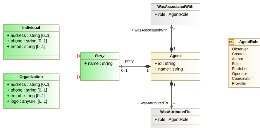
Figure 7: The relations between the Agent class within the Provenance Data Model (grey and yellow classes) with classes from the Dataset Metadata Model (green).
