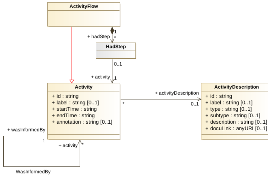
Figure 5: Details for Activity, ActivityDescription and ActivityFlow (see Section 2.2.4).
